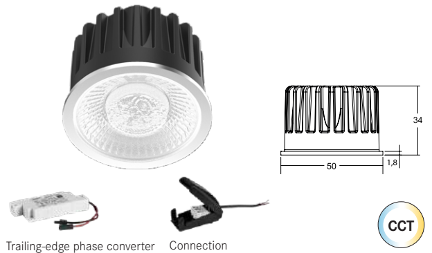
Trailing-edge phase converter
